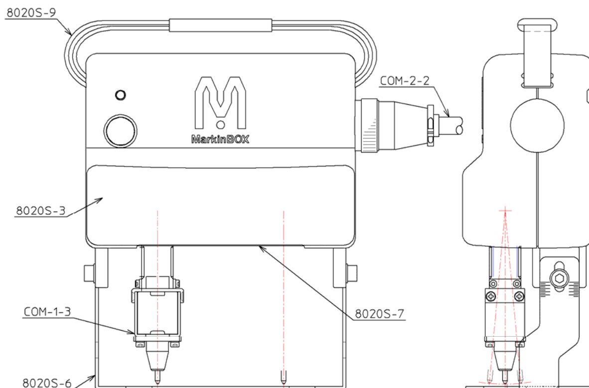
Complete set:8020S-1
